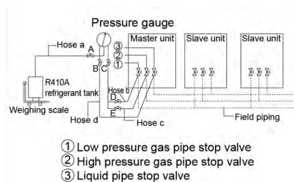
Figure 3-8.1: Charging refrigerant
